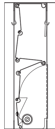
Closed Position (30DV)
