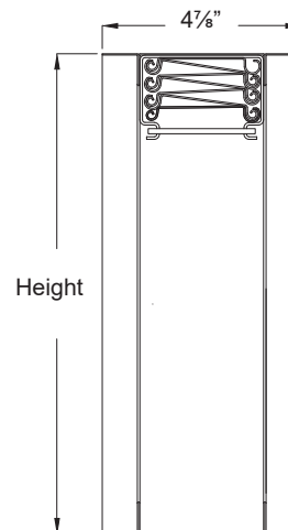
Open Position (30SV)
